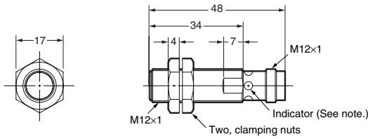
E2A-M12KS04-M1-□□/E2A-S12KS04-M1-□
