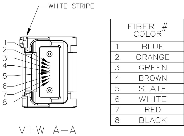
LIGHTRAY MPX CONNECTOR FIBER PATH
