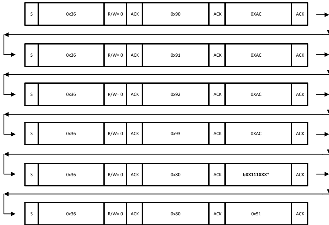
Figure 51. Pattern Generation Write Sequence
