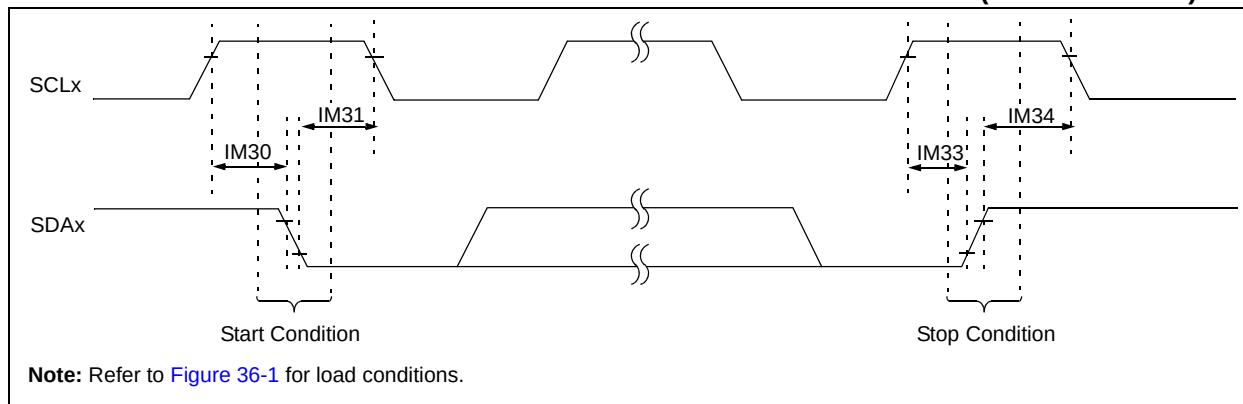
FIGURE 36-16: I2Cx BUS START/STOP BITS TIMING CHARACTERISTICS (MASTER MODE)
