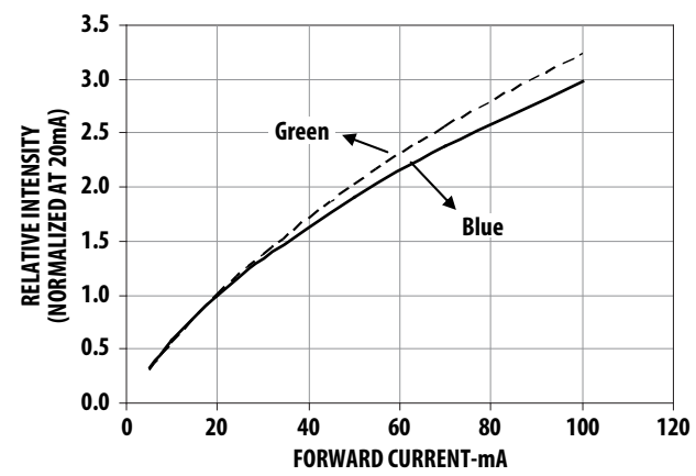
Figure 7 Relative Intensity vs. Forward Current
