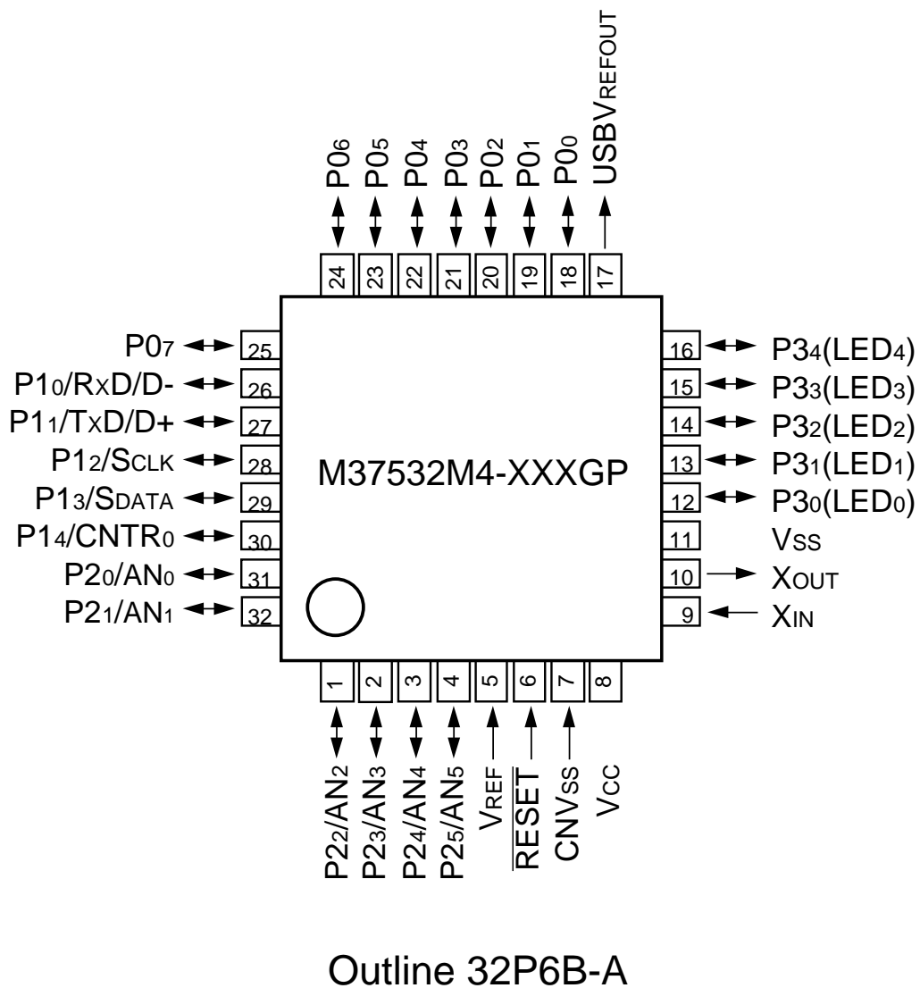
Fig. 2 Pin configuration of M37532M4-XXXGP
