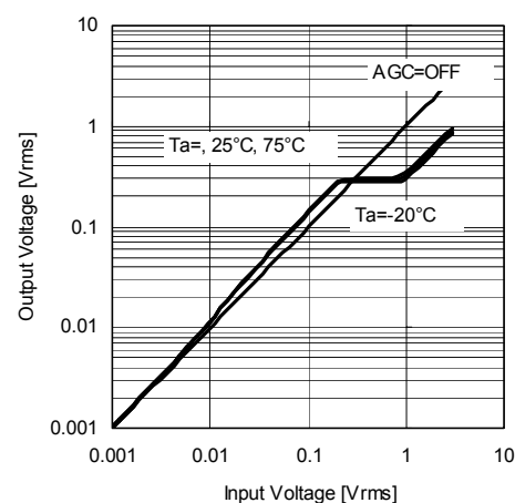
AGC Output Voltage vs. Input Voltage V_+=9\text{V} , R_L=47\text{k}\Omega , V_{in}(\text{A+Bch}) , f=1\text{kHz} , V_{out}(\text{Ach}) , \text{BW}=400\text{Hz}-30\text{kHz} , \text{VOL}=0\text{dB} , \text{BAL}=0\text{dB} , \text{AGC}=300\text{mV} , \text{BASS}=\text{TREB}=0\text{dB} , \text{BBE}=\text{OFF} , \text{Surround}=\text{OFF}
