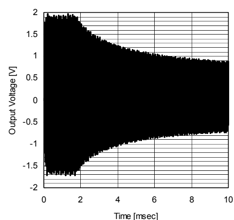
AGC Attack Time Response T_a=25^{\circ}\text{C} , V_+=9\text{V} , R_L=47\text{k}\Omega , V_{in}(\text{A+Bch}) , f=20\text{kHz} , V_{out}(\text{Ach}) , \text{BW}=400\text{Hz}-30\text{kHz} , \text{VOL}=0\text{dB} , \text{BAL}=0\text{dB} , \text{AGC}=300\text{mV} , \text{BASS}=\text{TREB}=0\text{dB} , \text{BBE}=\text{OFF} , \text{Surround}=\text{OFF}
