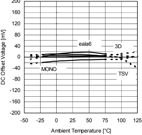
DC Offset Voltage vs. Ambient Temperature (Surround) V+=9V, RL=47kΩ, Bypass : VOL=0dB, BAL=0dB, AGC=OFF, BASS=TREB=0dB, BBE=OFF
