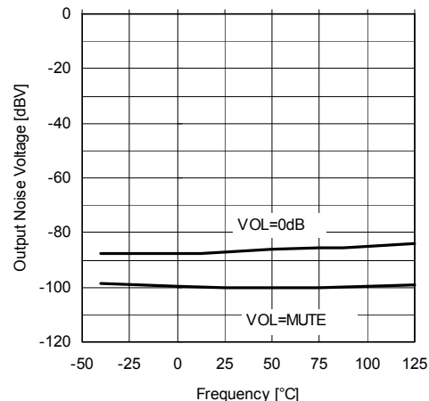
Output Noise Voltage (OUT) vs. Frequency V_+=9\text{V} , R_L=47\text{k}\Omega , \text{BAL}=0\text{dB} , \text{AGC}=\text{OFF} , \text{BASS}=\text{TREB}=0\text{dB} , \text{BBE}=\text{OFF} , \text{Surround}=\text{OFF}
