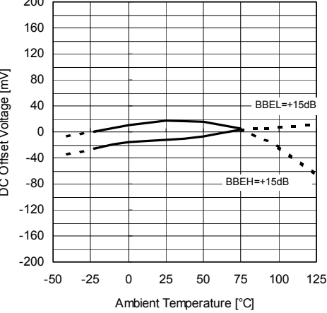
DC Offset Voltage vs. Ambient Temperature (BBE) V+=9V, RL=47kΩ, Bypass : VOL=0dB, BAL=0dB, AGC=OFF, BASS=TREB=0dB, Surround=OFF
