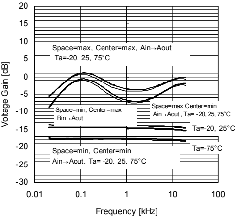
Voltage Gain vs. Frequency (3D) Ta=25°C, V+=9V, RL=47kΩ, Vin=0.1Vrms, VOL=0dB, BAL=0dB, BASS=TREB=0dB, AGC=OFF, BBE=OFF, Surround=3D
