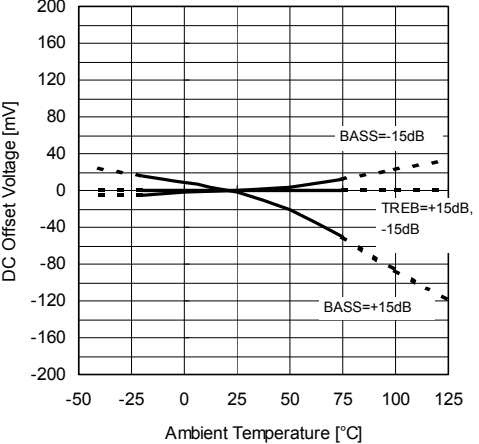
DC Offset Voltage vs. Ambient Temperature (TONE) V+=9V, RL=47kΩ, Bypass : VOL=0dB, BAL=0dB, AGC=OFF, BBE=OFF, Surround=OFF
