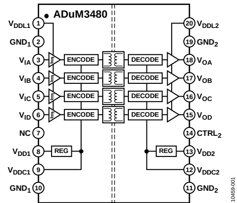
Figure 1. ADuM3480
