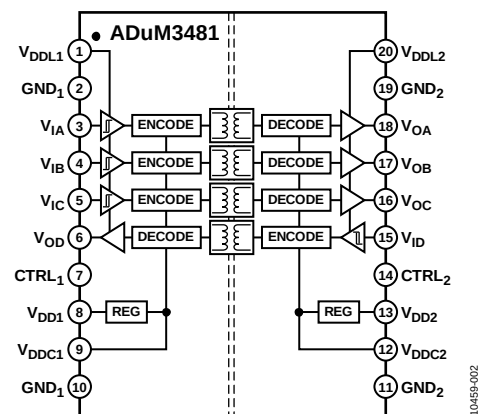
Figure 2. ADuM3481
