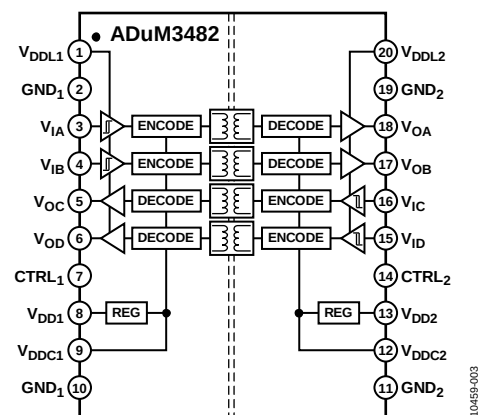
Figure 3. ADuM3482
