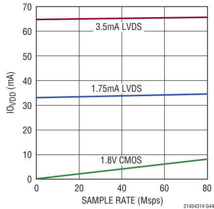
LTC2143-14: I_{O_VDD} vs Sample Rate, 5\text{MHz} , -1\text{dBFS} , Sine Wave Input on Each Input
