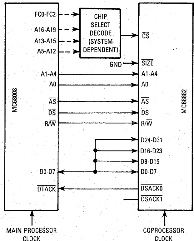
Figure 15. 8-Bit Data Bus Peripheral Processor Connection
