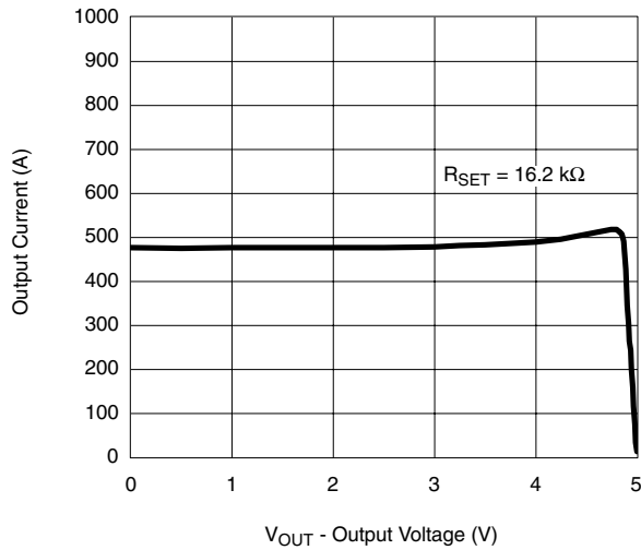
Output Current vs. V_{\text{OUT}}
