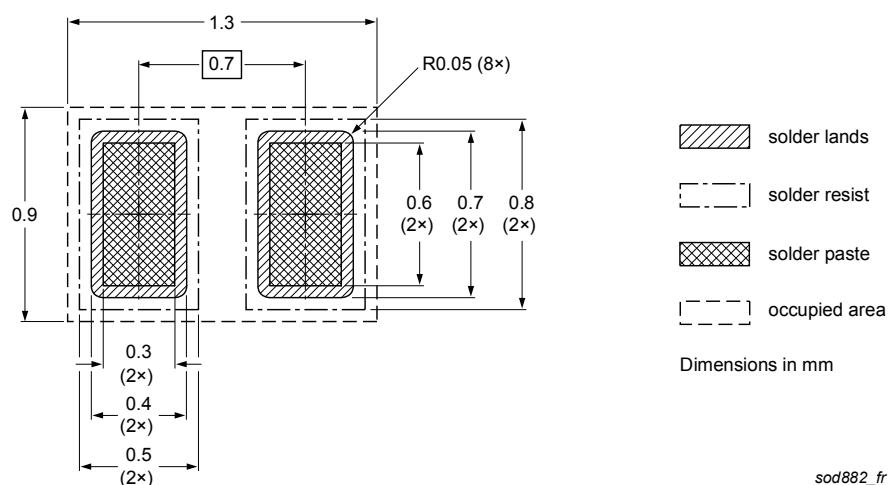
Fig. 12. Reflow soldering footprint for DFN1006-2 (SOD882)
