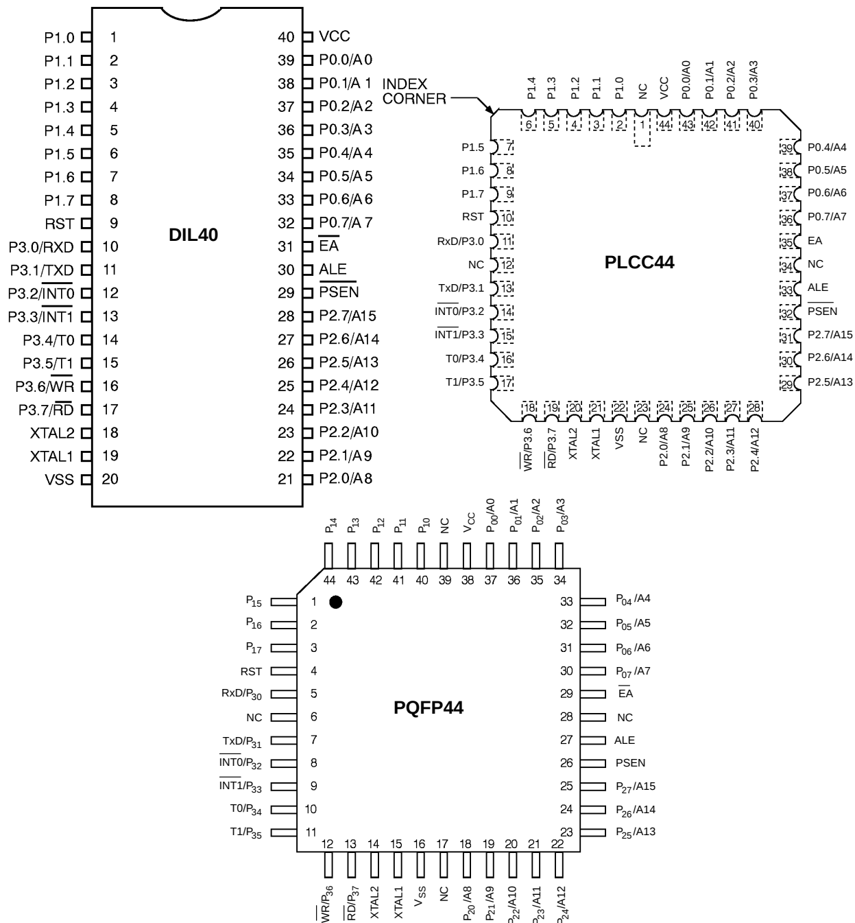
Figure 2. Pin Configuration
