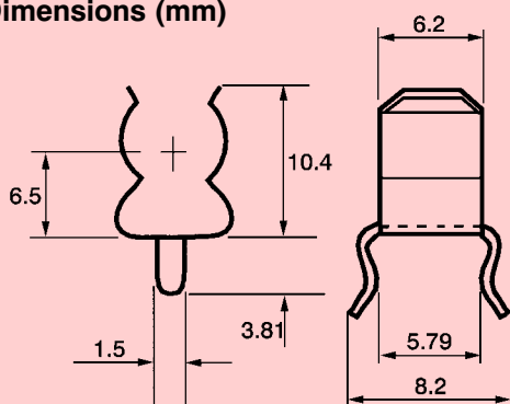
Dimensions (mm)
