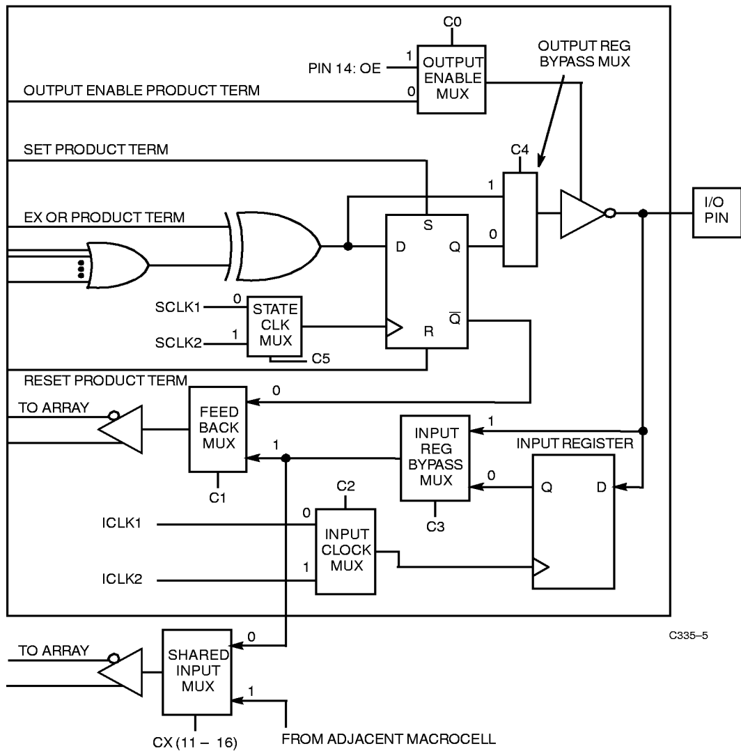
Figure 2. CY7C335 Input/Output Macrocell
