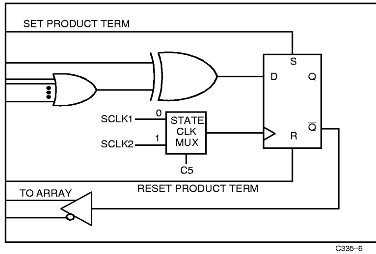
Figure 3. CY7C335 Hidden Macrocell
