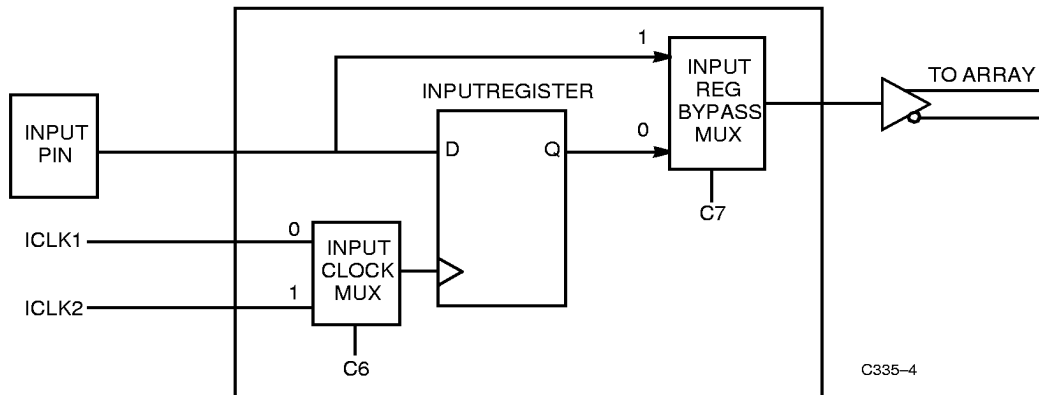
Figure 1. CY7C335 Input Macrocell
