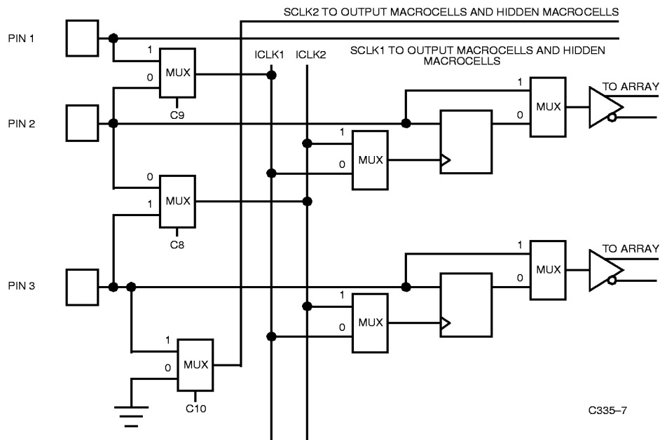
Figure 4. CY7C335 Input Clocking Scheme
