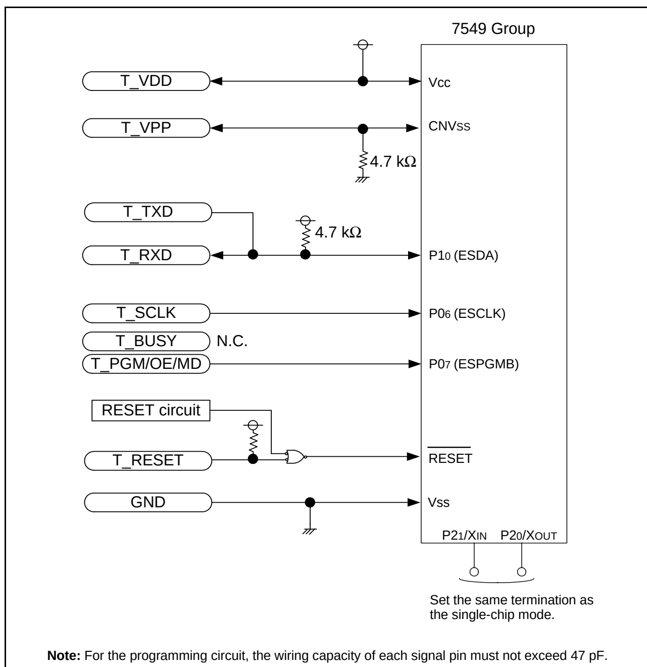
Fig 71. When using programmer of Suissei Electronics System Co., LTD, connection example
