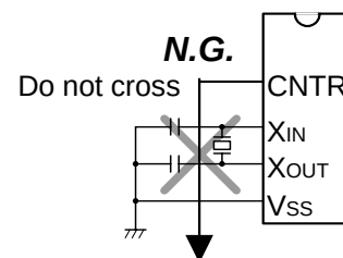
Fig 77. Wiring for a large current signal line/Writing of signal lines where potential levels change frequently
