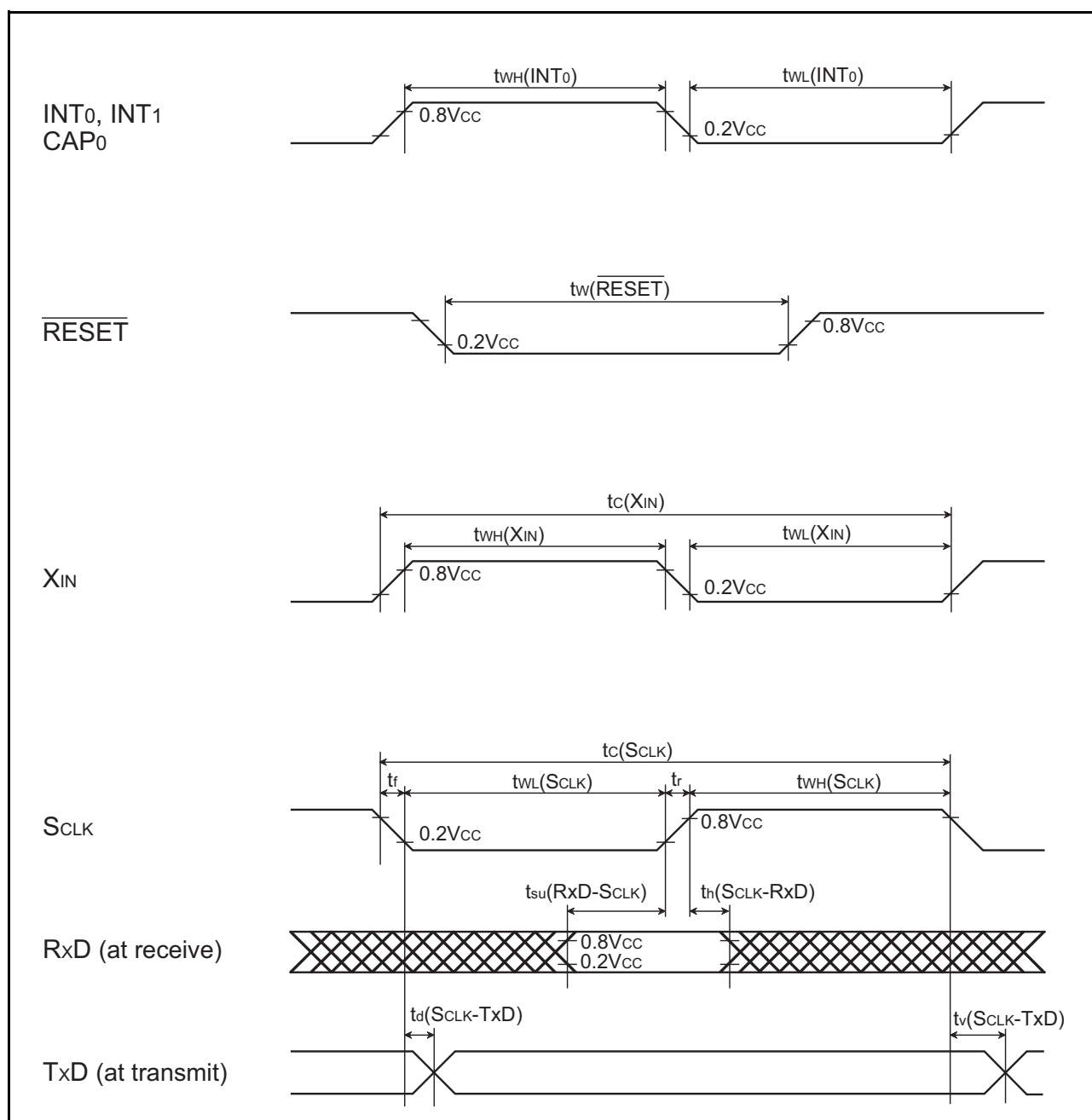
Fig 85. Timing chart
