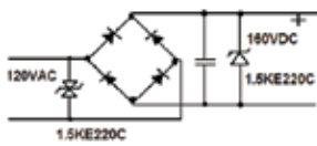
TVSD in Bridge Rectifier Protection
