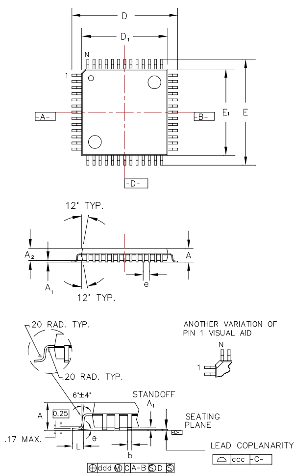
Figure C-1. Stellaris LM3S5951 100-Pin LQFP Package Dimensions
