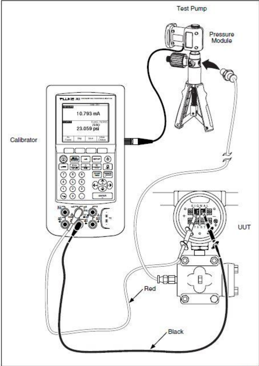
Figure 2. Using the Pump
