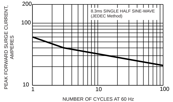
FIG. 4 - MAXIMUM NON-REPETITIVE PEAK FORWARD SURGE CURRENT UNIDIRECTIONAL ONLY
