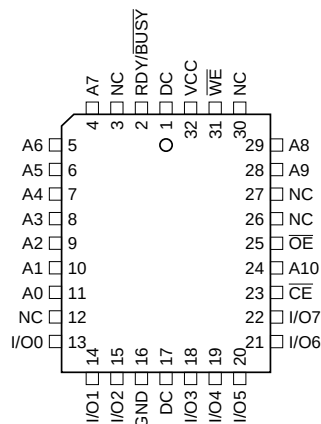
PLCC Top View
