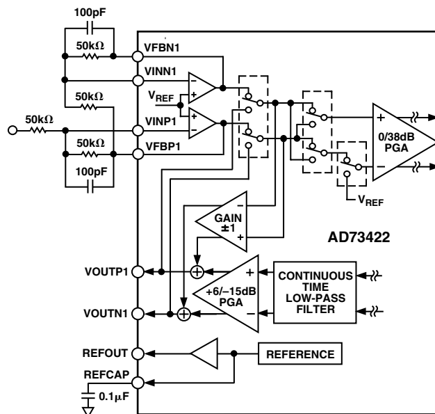
Figure 30. Single-Ended-to-Differential Conversion On Analog Input
