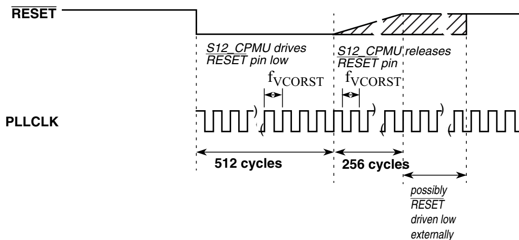
Figure 10-34. RESET Timing
