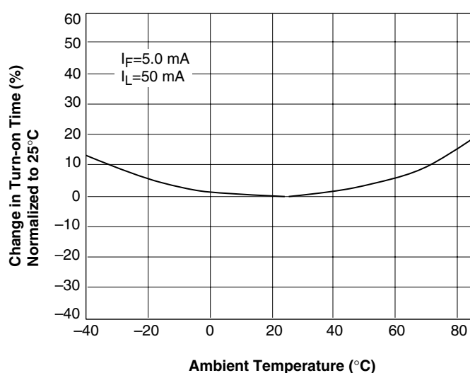
Figure 9. Turn-on Time vs. Temperature
