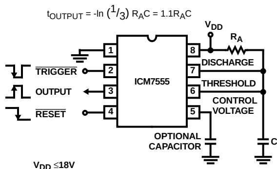
FIGURE 3. MONOSTABLE OPERATION
