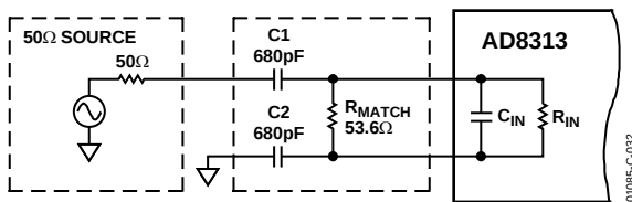
Figure 32. A Simple Broadband Resistive Input Termination
