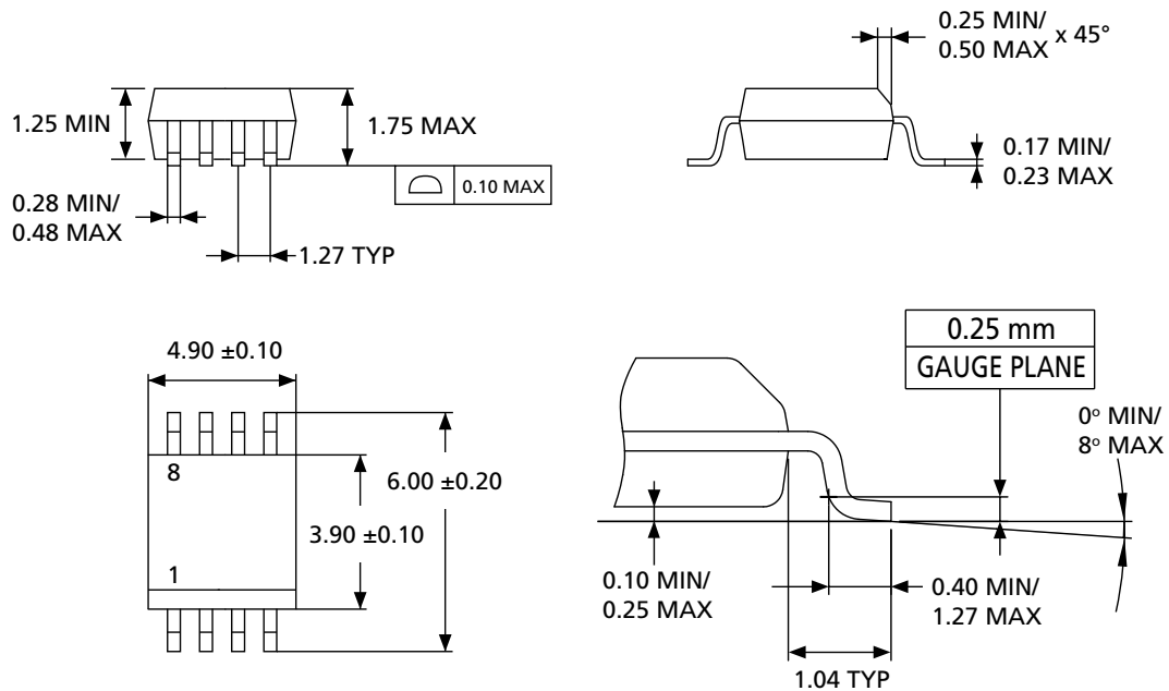
Figure 27: SO8N 150 mils Body Width
