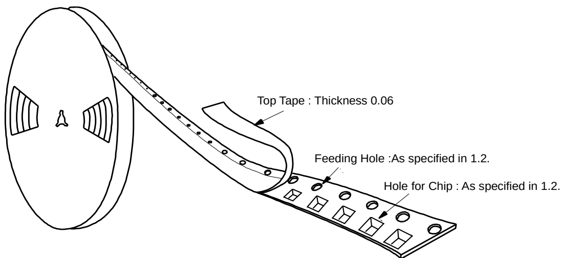
Fig.3 Taping Diagram
