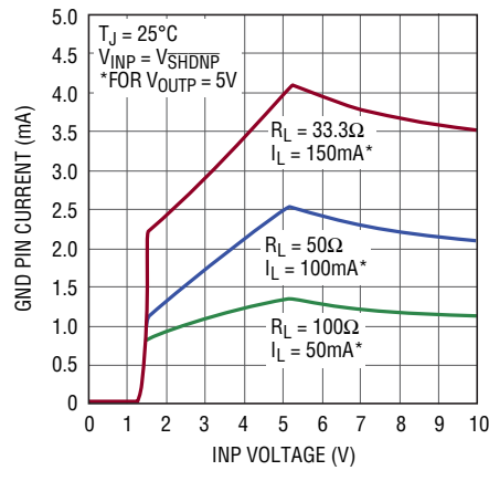
LT3032-5 Positive Side GND Pin Current
