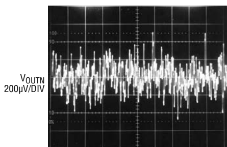
OUTN, 10Hz to 100kHz Output Noise, C BYPN = 0
