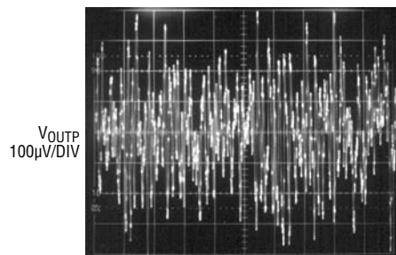
OUTP 10Hz to 100kHz Output Noise C BYP = 0
