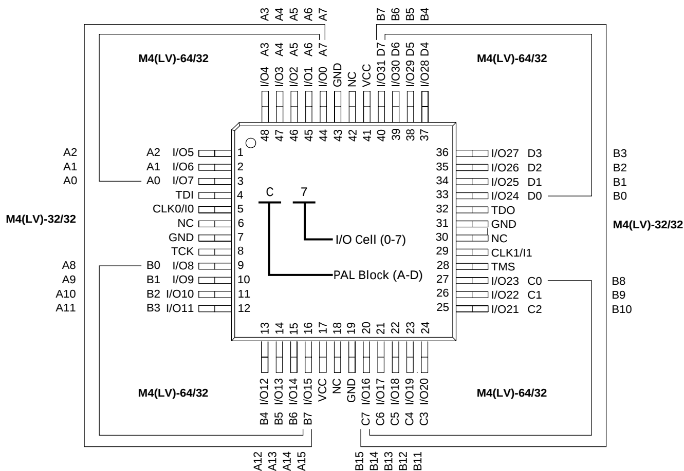
48-Pin TQFP
