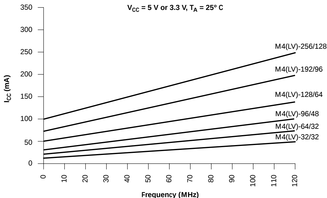
Figure 19. MACH 4 I_{CC} Curves at Low Power Mode
