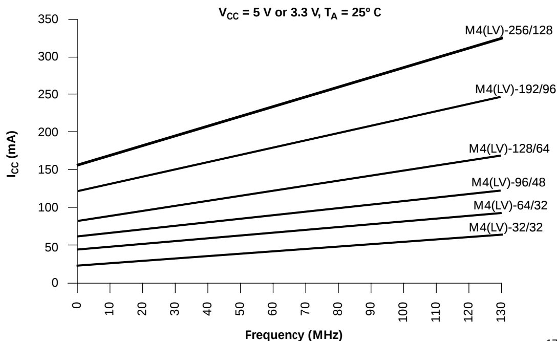
Figure 18. MACH 4 I_{CC} Curves at High Speed Mode
