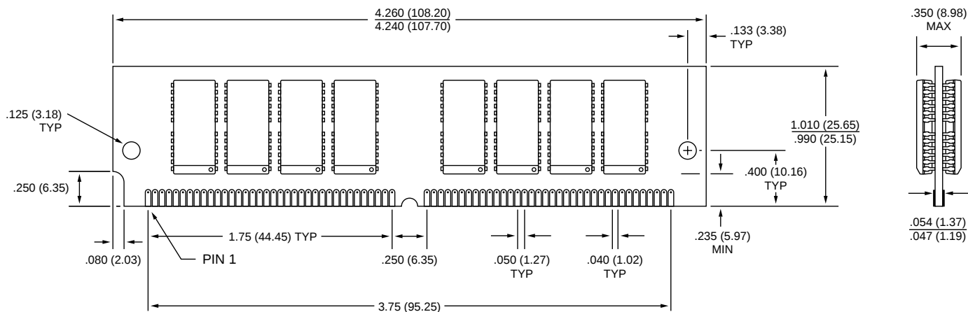
72-Pin SIMM (32MB)
