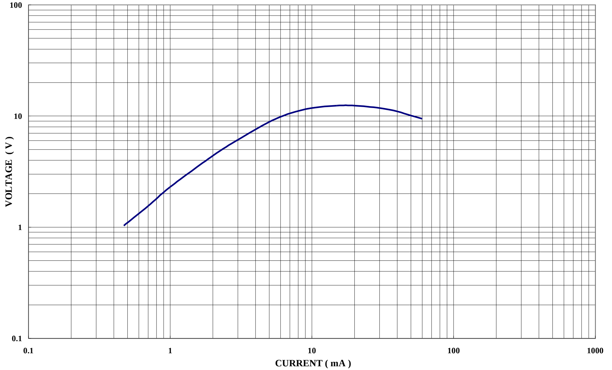
V-I Curve ( Nominal ) Part No. : TDC05C225
