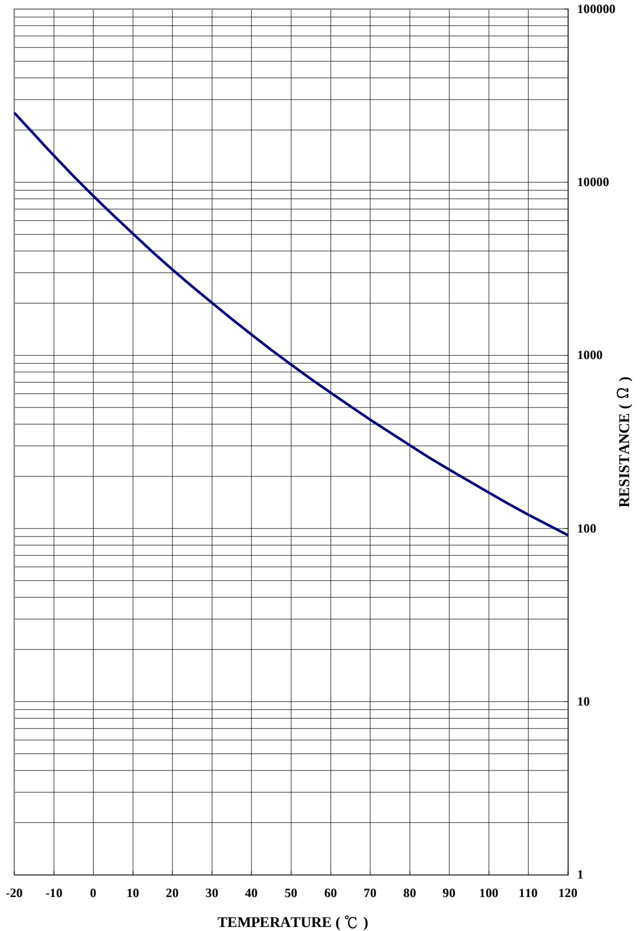
R-T Curve ( Nominal ) Part No : TDC05C225
