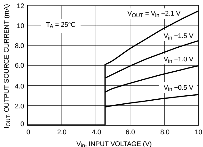
Figure 20. NCP300L Series 4.5 V Reset Output Source Current versus Input Voltage
