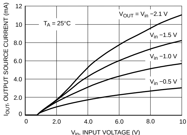
Figure 18. NCP300L Series 0.9 V Reset Output Source Current versus Input Voltage
