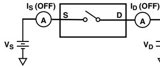
Test Circuit 2. Off Leakage
