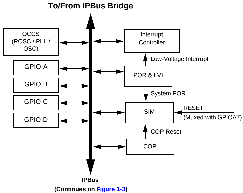
Figure 1-2 Peripheral Subsystem
