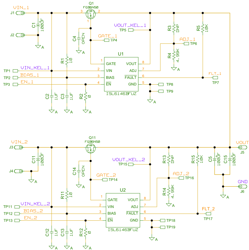
FIGURE 59. ISL6146BEVAL1Z SCHEMATIC
