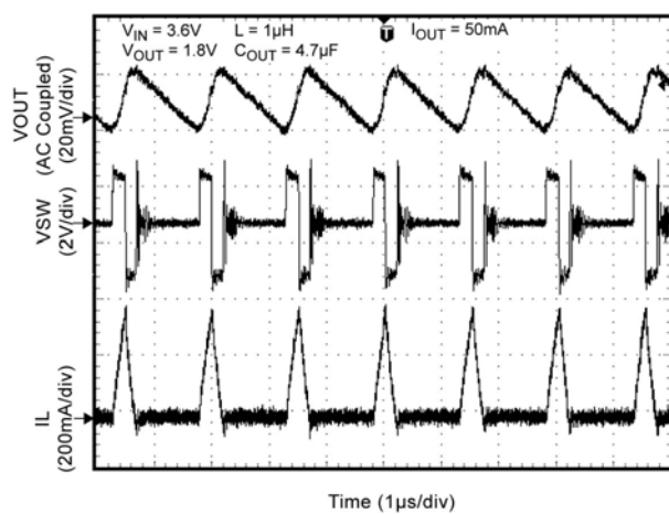
Switching Waveform
