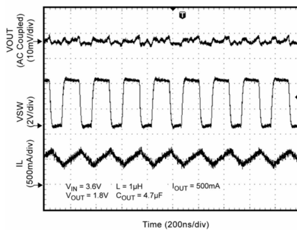
Switching Waveform
