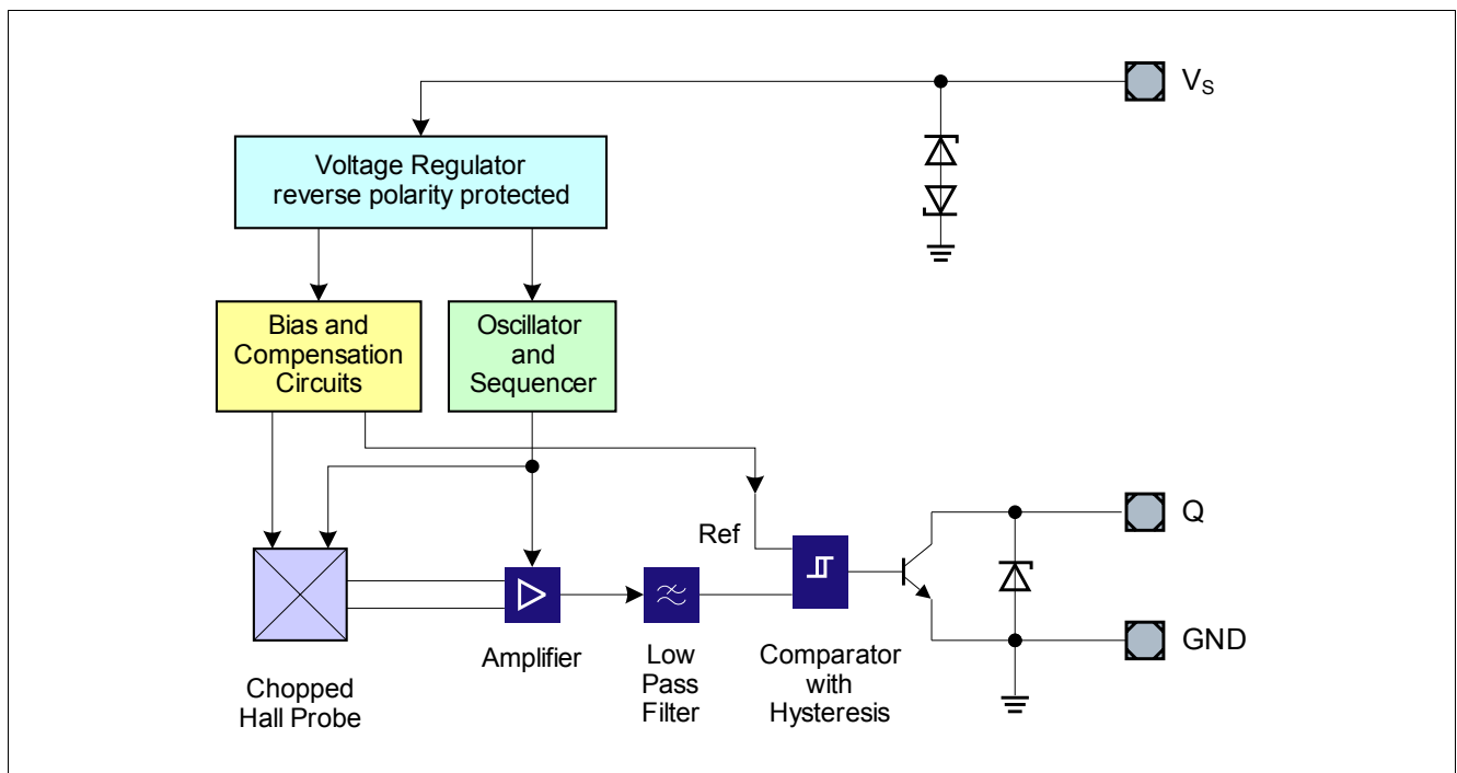
Figure 2 TLV4946xy Block Diagram
