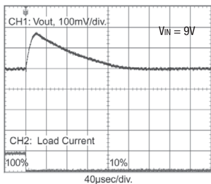
7805SR-C 100% to 10% Load Step
