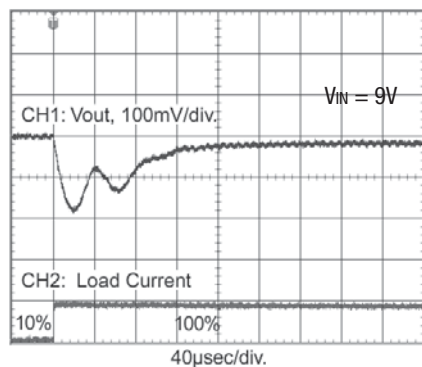
7805SR-C 10% to 100% Load Step
