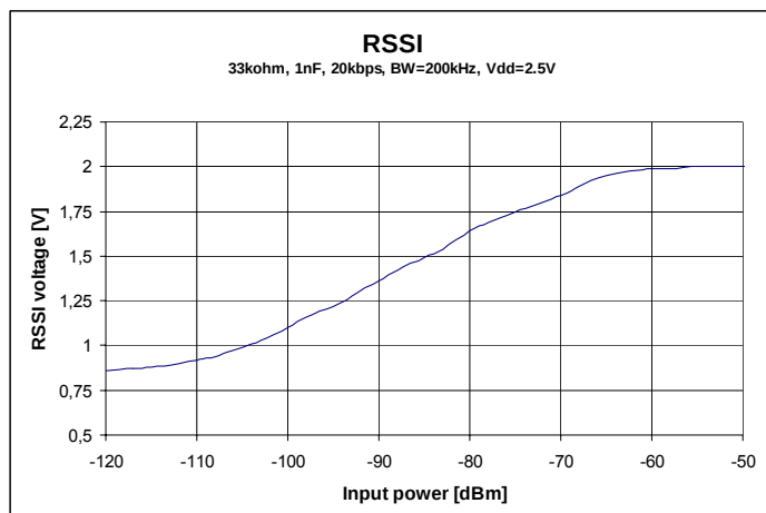
Figure 10. RSSI Voltage
