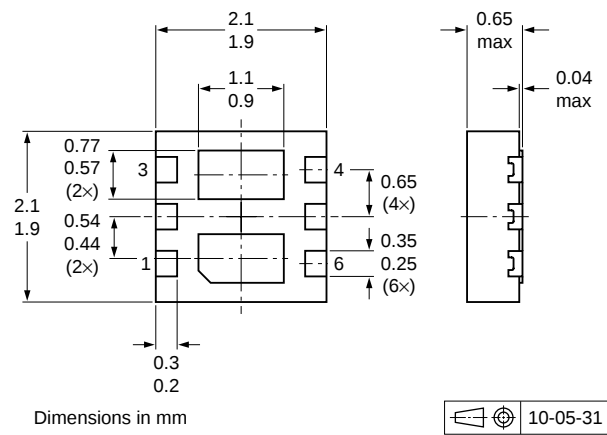
Fig 18. Package outline SOT1118 (HUSON6)
