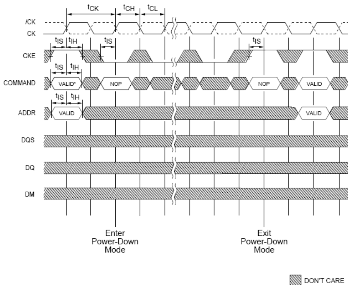
Figure 39 - POWER-DOWN MODE
