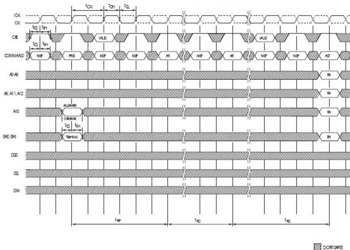
Figure 40 - AUTO REFRESH MODE
