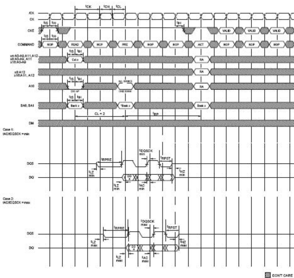
Figure 43 - READ - WITH AUTO PRECHARGE
