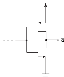
Figure 3-5: \overline{CD} Circuit
