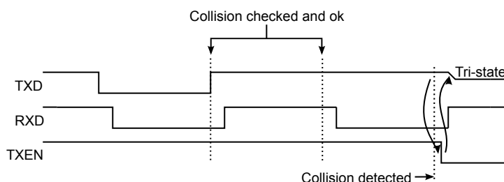
Figure 31-17. Collision Detected
