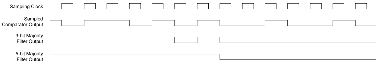
Figure 40-8. Single-Shot Filtering
