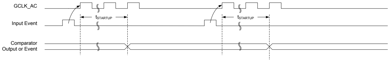
Figure 40-11. Single-Shot SleepWalking
