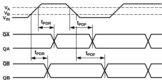
Figure 2. Timing Diagram I
