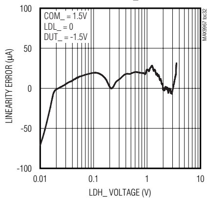
ACTIVE-LOAD LINEARITY ERROR I DUT- vs. LDH -
