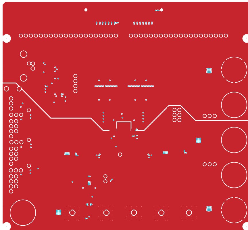
Figure 6. Component Side
