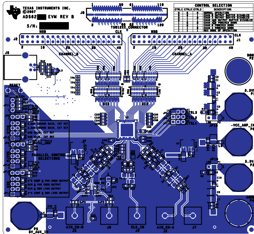
Figure 5. Top Silkscreen
