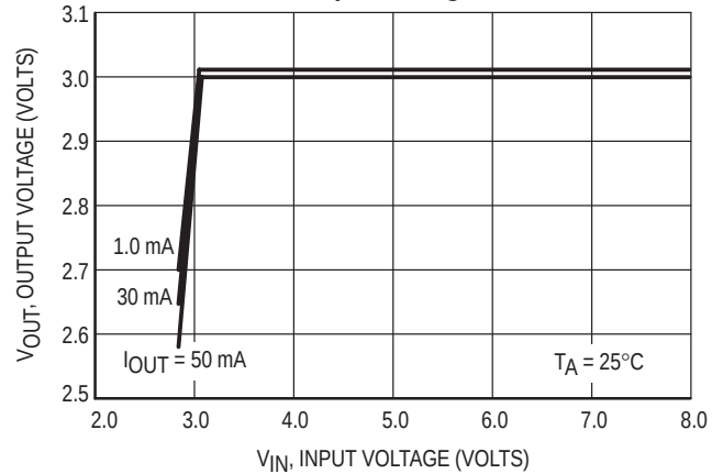
Figure 10. MC78PC30 Output Voltage versus Input Voltage
