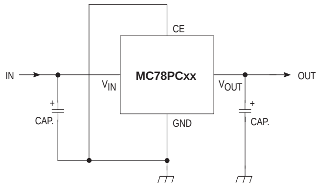
Figure 47. Typical Application
