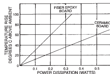
POWER DISSIPATION
