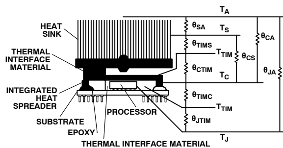
Figure 66. Thermal Model
